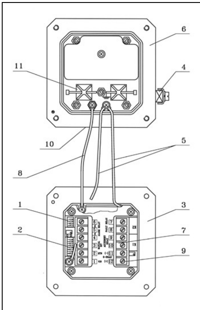
Figure 5. UV/IR Flame Detector with Cover Removed
