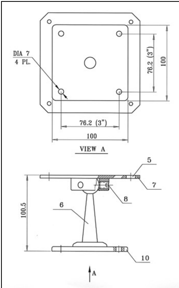
Figure 4.b. Swivel Mount Assembly
