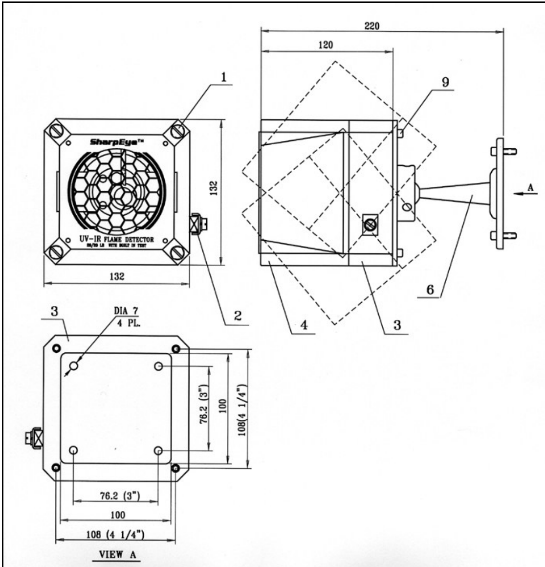
Figure 4.a. U/IR Detector and Swivel Mount Assembly
