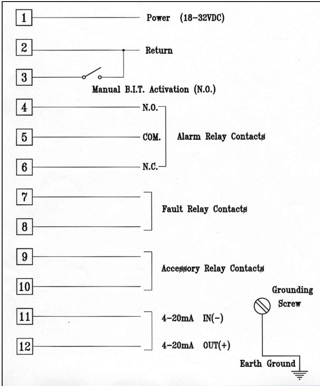
Figure 7. Flame Detector Assembly - Wiring Diagram
