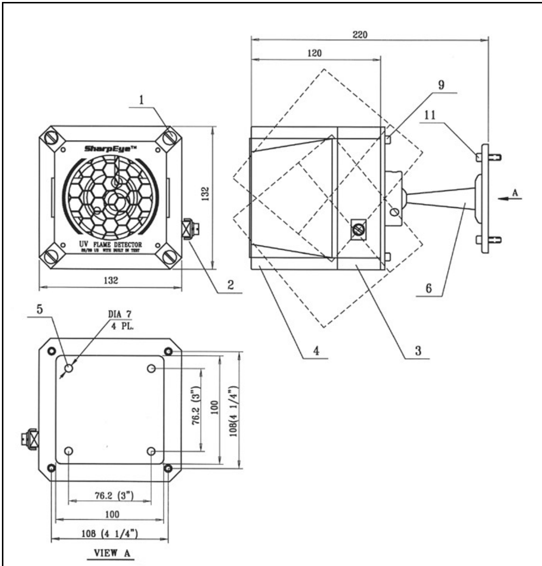
Figure 4.a. UV Detector and Swivel Mount Assembly
