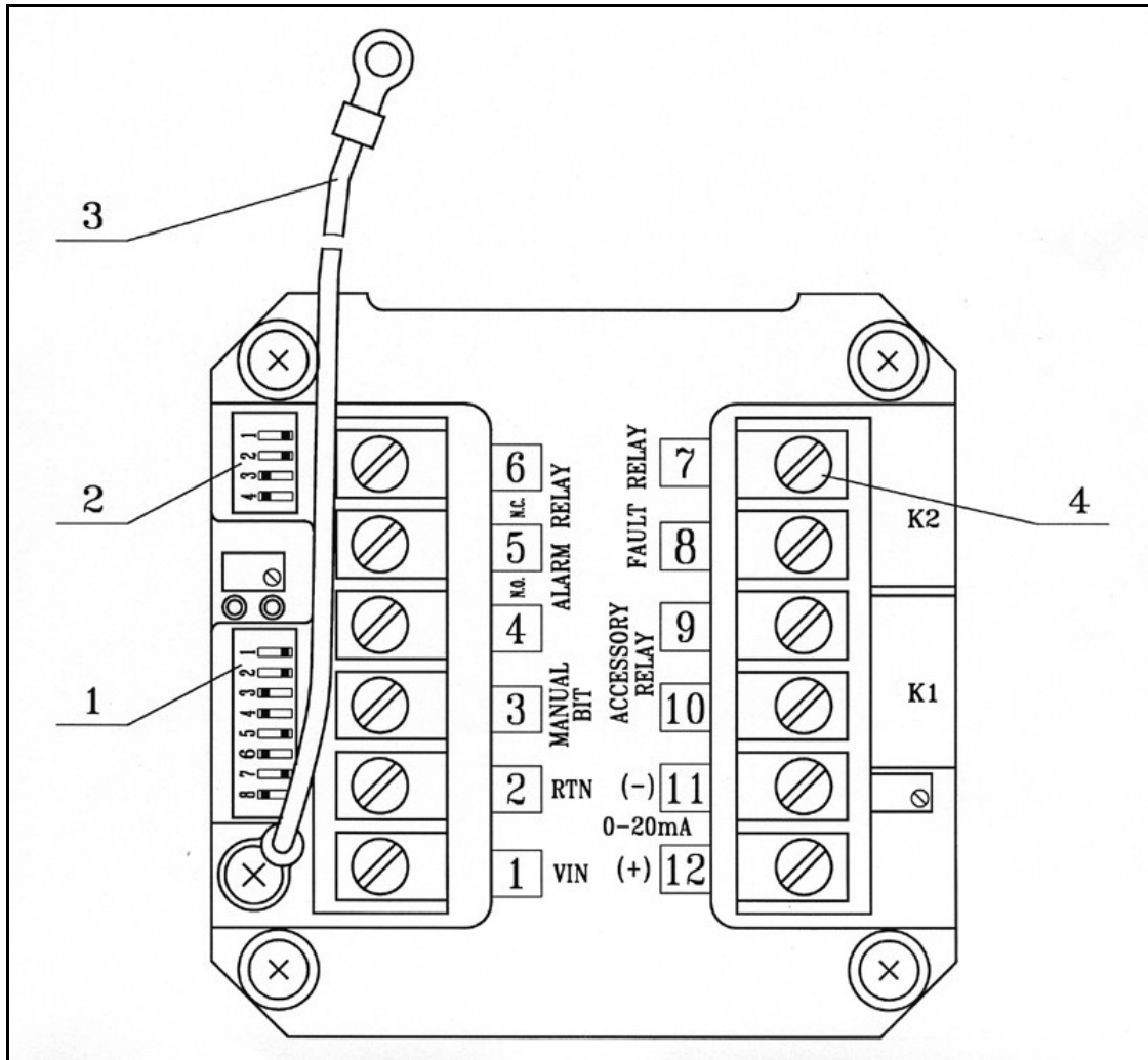
Figure 6. Terminal Board Configuration
