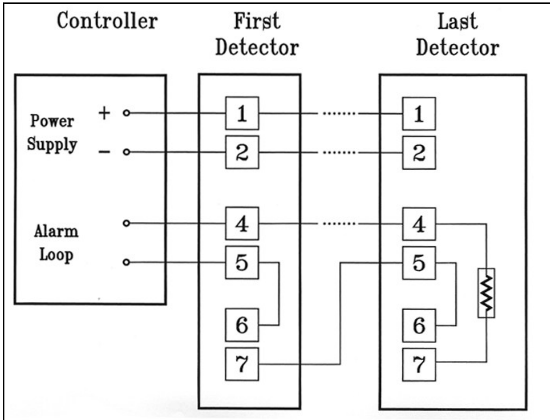
Figure 8. Typical Wiring Diagram for Four-Wire Controller
