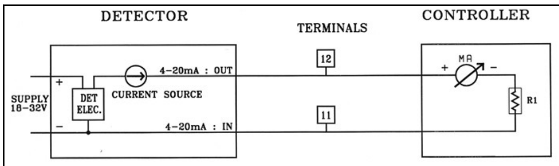
Figure 9. Wiring Diagram for 4-20mA
