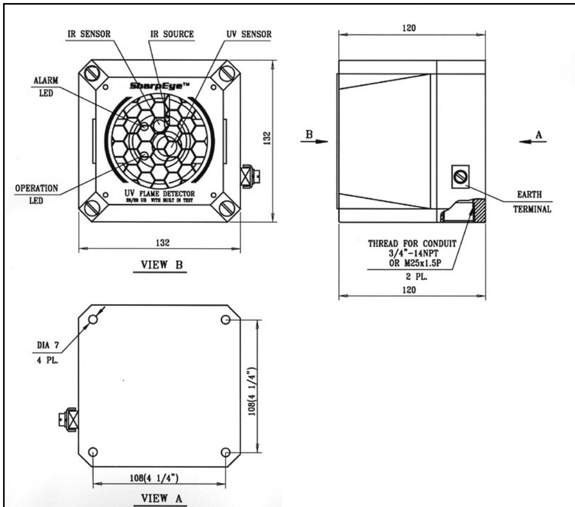
Figure 1. Flame Detector Assembly - Outline Drawing
