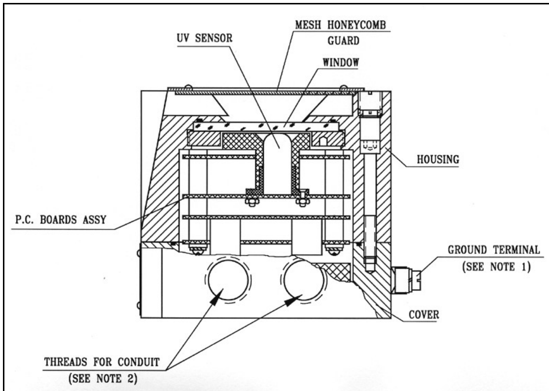
Figure 2. Flame Detector Assembly - Schematic Section
