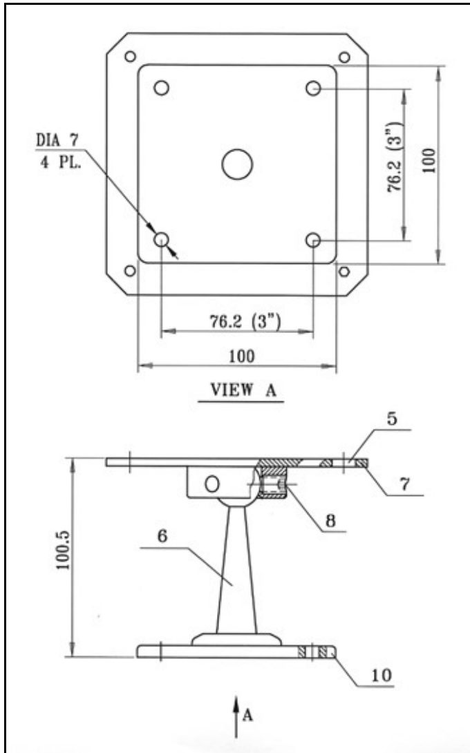
Figure 4.b. Swivel Mount Assembly
